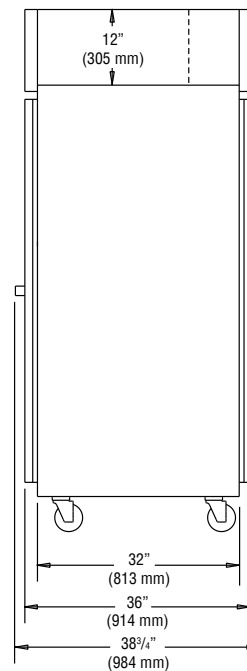
RIGHT VIEW
