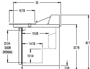
C-Top Side View
