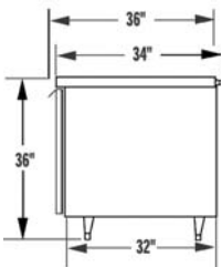
DLFB-SS SIDE VIEW
