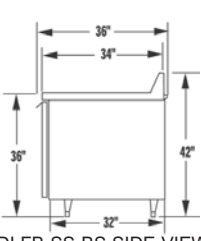
DLFB-SS-BS SIDE VIEW
