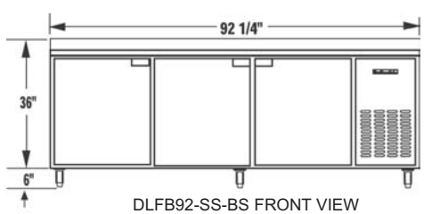
DLFB92-SS-BS FRONT VIEW
