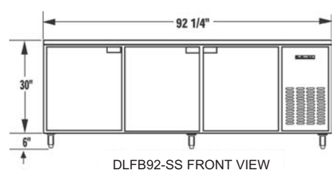
DLFB92-SS FRONT VIEW
