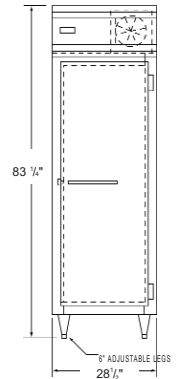
DL1FE-SS FRONT VIEW
