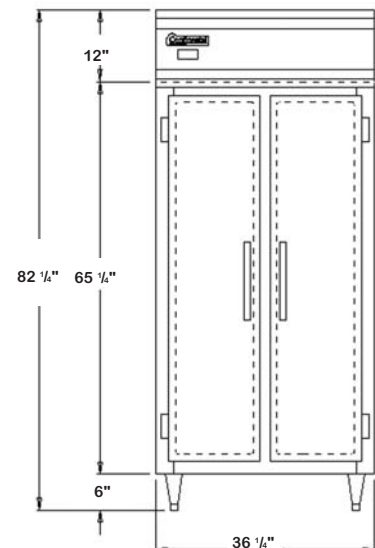
DL2RSE FRONT VIEW
