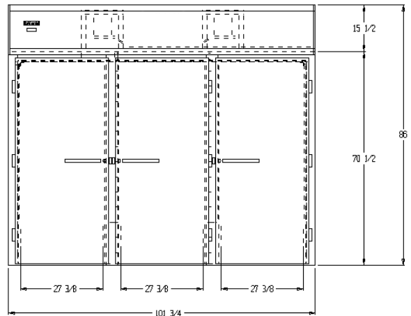
DL3WI-SS FRONT VIEW
